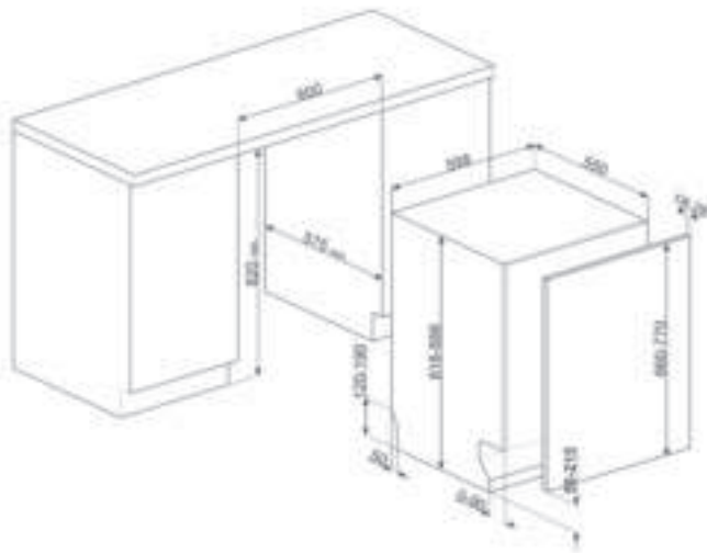
LAVASTOVIGLIE LARGHEZZA 60 CM: STL7324AQLLW, STL7324AQL, STL7322AL, STL7322BQL, STL7322BL, STL7332CL, STL7352C, STL7252C, ST7272D
