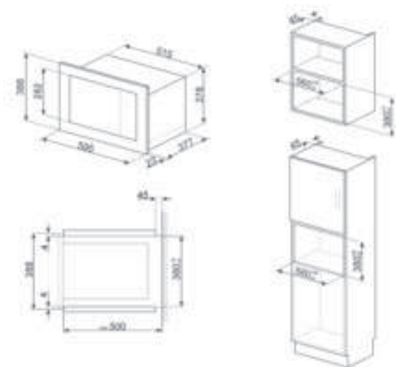
MICROONDE: FMI625CN, FMI125G, FMI125N
